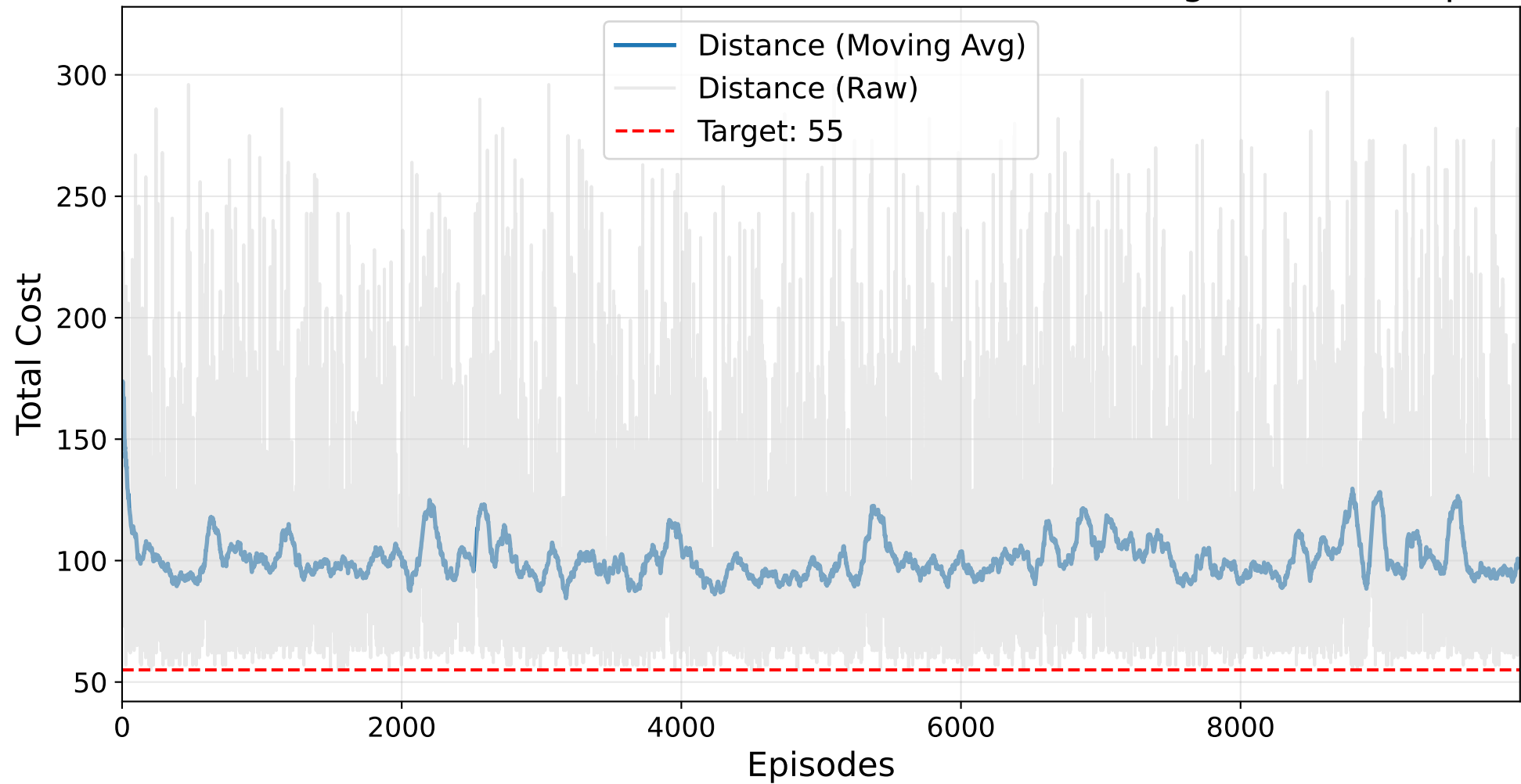
Final GAUSSIAN PROCESS Masked AutoRL-SOP Training - br17.12.sop
